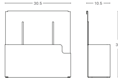
AC-05 Dominium Paper Holder
