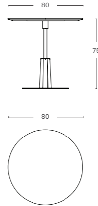
TL-02 Exilium Round Table
